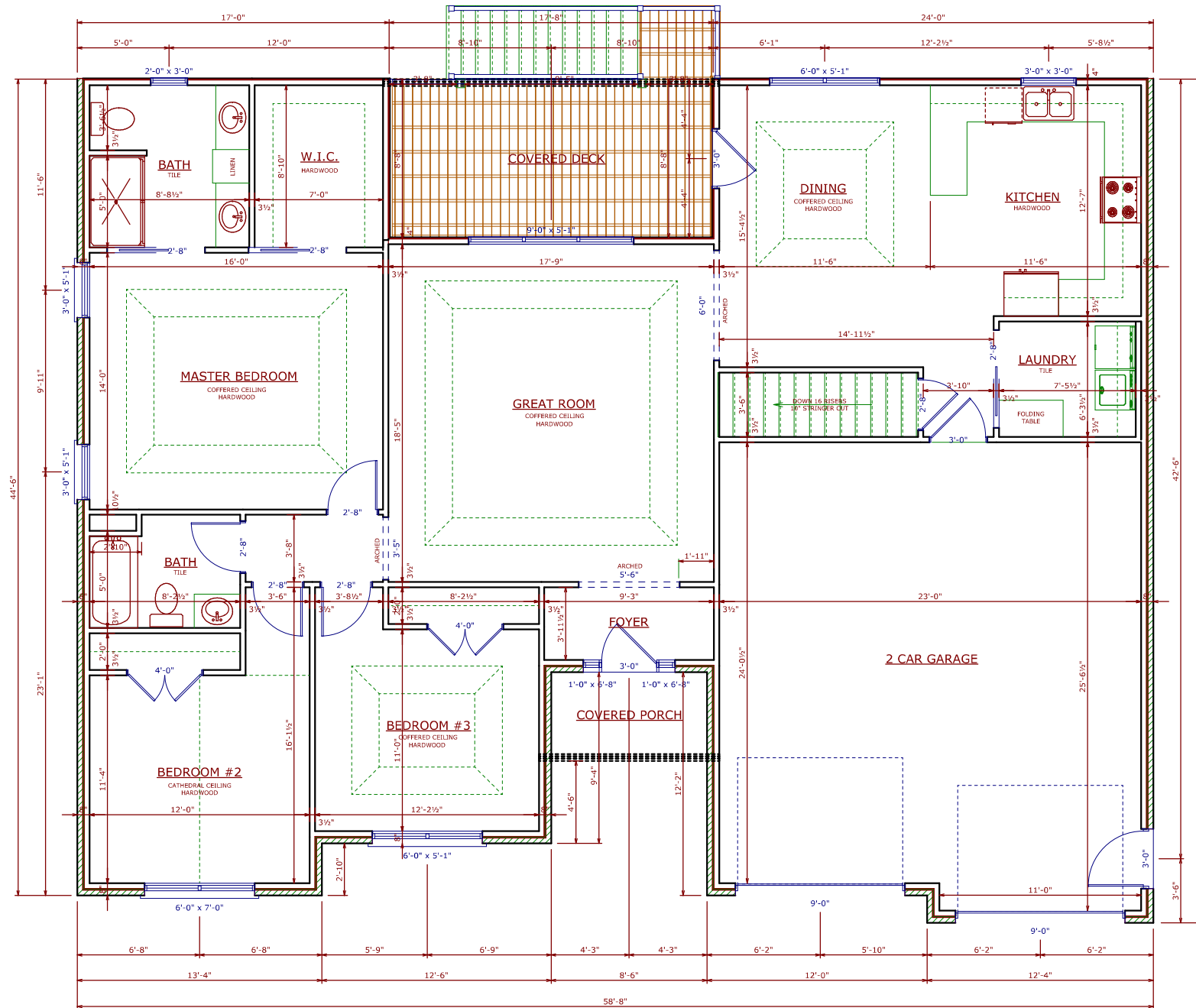
MAIN FLOOR PLAN NOTE: 8' WALL HEIGHT UNLESS NOTED
