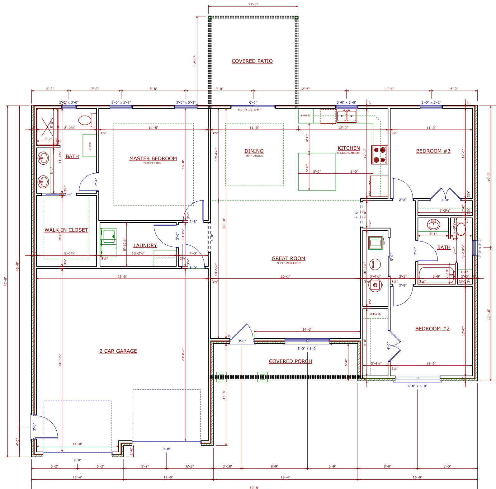
MAIN FLOOR PLAN NOTE: 8' CEILING HEIGHT UNLESS NOTED
