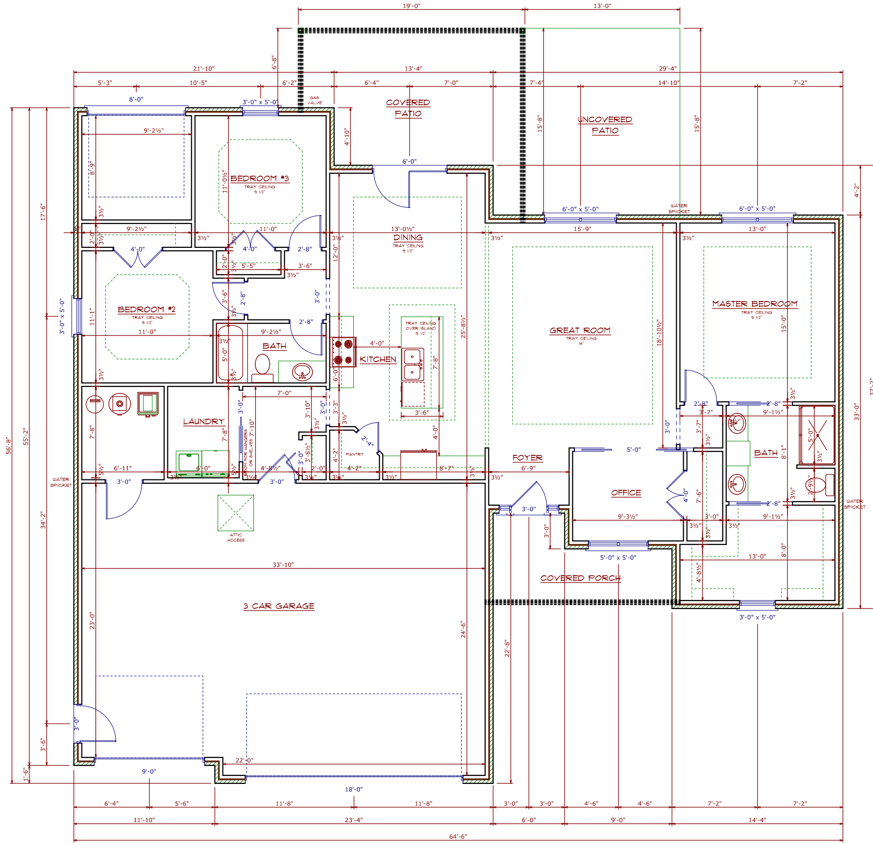
MAIN FLOOR PLAN NOTE: 8' WALL HEIGHTS UNLESS NOTED
