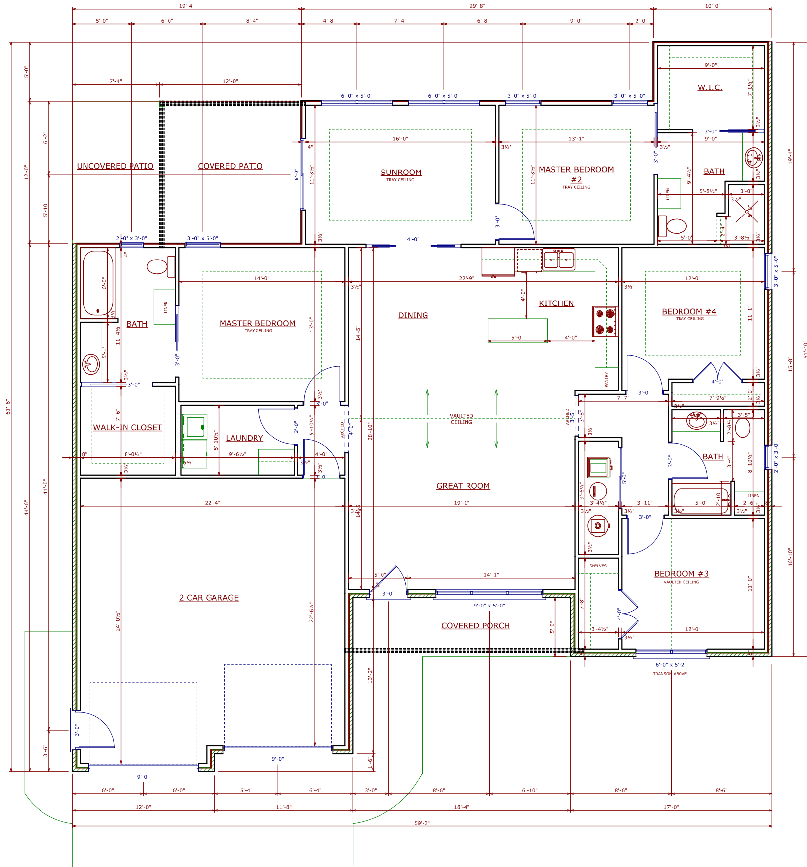
MAIN FLOOR PLAN NOTE: 8' CEILING HEIGHT UNLESS NOTED
